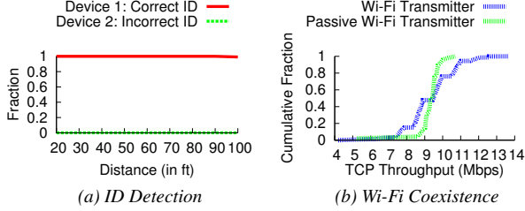
Figure 17: Passive Wi-Fi network performance.
