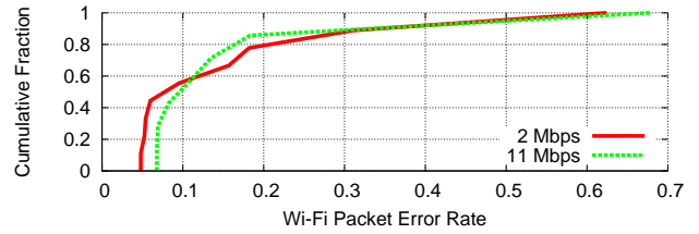
Figure 11—Wi-Fi packet error rate. We measured packet error rate for backscatter-generated Wi-Fi packets at both 2 and 11 Mbps.
