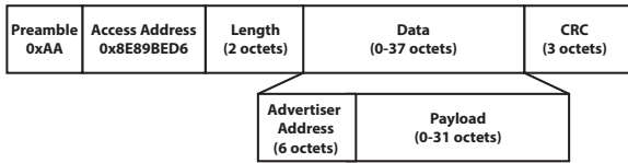
Figure 5—Structure of a Bluetooth advertising packet.
