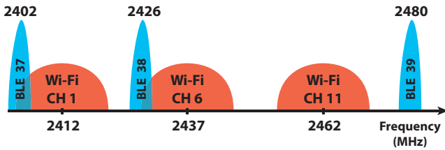
Figure 3—Wi-Fi versus Bluetooth. The blue frequencies represent the three Bluetooth advertising channels and the red frequencies represent the three Wi-Fi channels.
