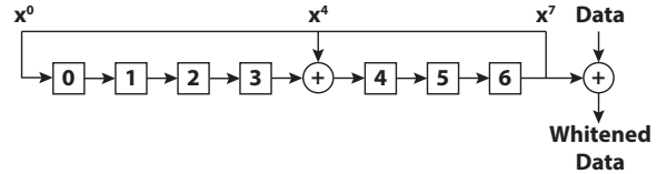
Figure 4—Shift registers used in Bluetooth to perform data whitening.
