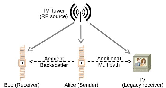
Figure 1—Ambient Backscatter: Communication between two battery-free devices. One such device, Alice, can backscatter ambient signals that can be decoded by other ambient backscatter devices. To legacy receivers, this signal is simply an additional source of multi-path, and they can still decode the original transmission.
