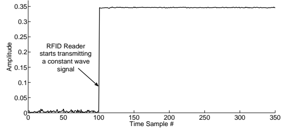
(b) Captured RFID Reader Signal
