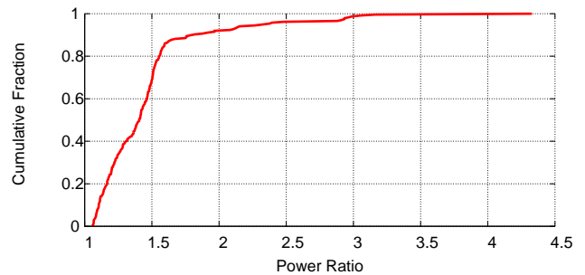
Figure 8—Performance of an ambient backscattering transmitter: The x-axis plots a CDF of the ratio of the average power received during the reflecting and non-reflecting states of the backscattering transmitter. The CDF is taken across multiple positions in both indoor/outdoor and near/far scenarios.
